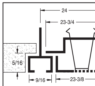
Model 3PD-D 9/16" NARROW SLOT
