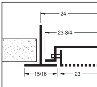
Model 3PD-L Lay-In, 15/16" (shown)
