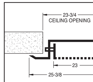
Model 3PD-F SURFACE MOUNTED
