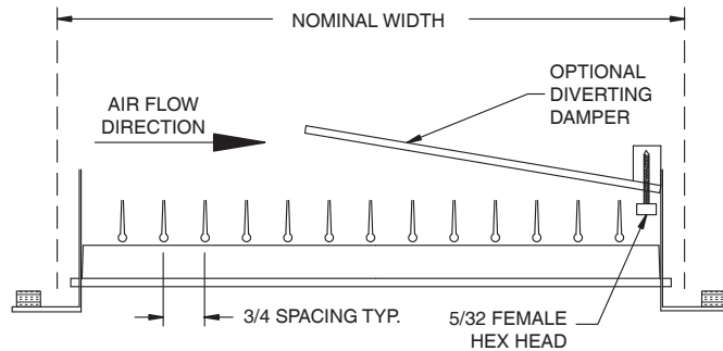
Model ECO20, Front Blade Direction Long (L) Shown
