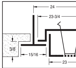
Model PAC-T Tegular, 15/16" (shown)
