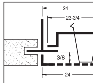
Model PAC-C Concealed Spline
