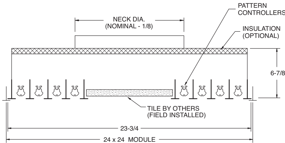
MODEL QL-S/L - Lay-In T-Bar (4 Slot Shown)
