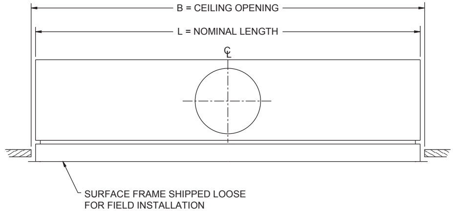
FACE VIEW OF SURFACE FRAME FOR ONE WAY PATTERNS
