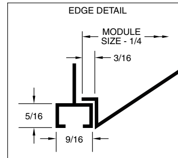
Model TMW - 9/16" Narrow Slot
