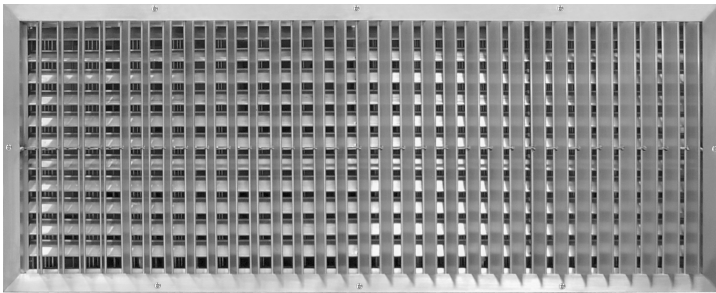
Model XW/S/OB Shown Vertical Face Blades with Opposed Blade Damper
