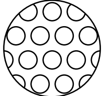
FACE PLATE PATTERN 3/16" DIAMETER HOLES ON 1/4" STAGGERED CENTERS
