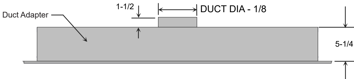
SECTION A - A (EDGE DETAIL)
