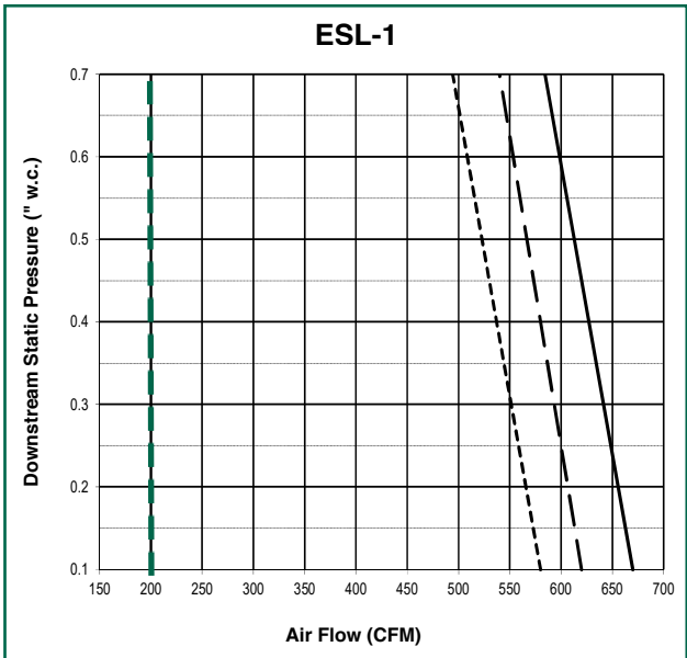
Graph 1: Fan Performance Data: Cooling Only, Electric Heat, 1&2 Row Hot Water Coil 120 / 208 / 240 / 277 VAC, 1Ø, 60 Hz
