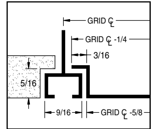
9/16 NARROW SLOT
