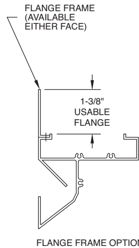
FLANGE FRAME OPTION
