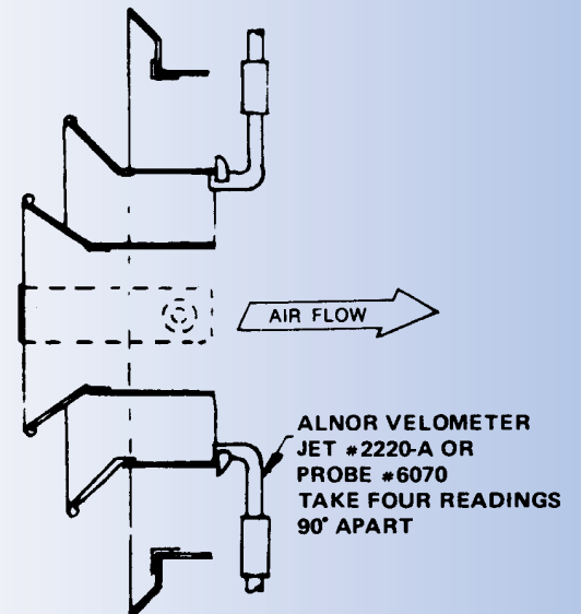
JET PATTERN SECTION A-A ROTATED
