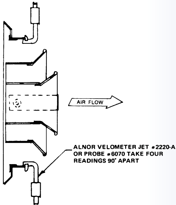
DIFFUSER PATTERN SECTION A-A ROTATED
