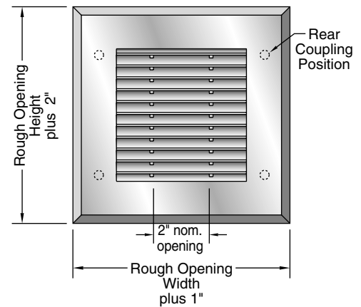
FRONT SECTION
